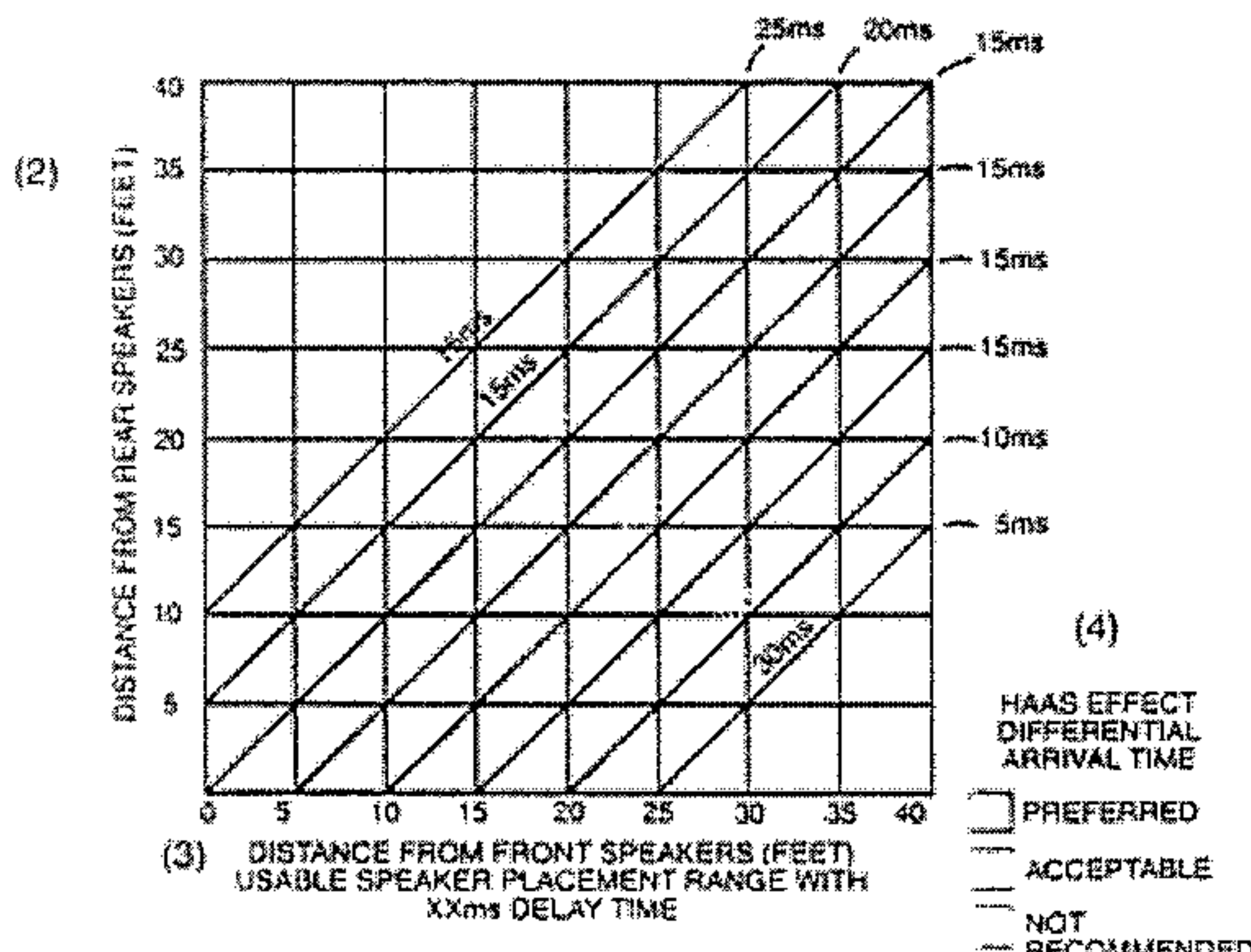
Figure 5. DOLBY DELAY (1)
