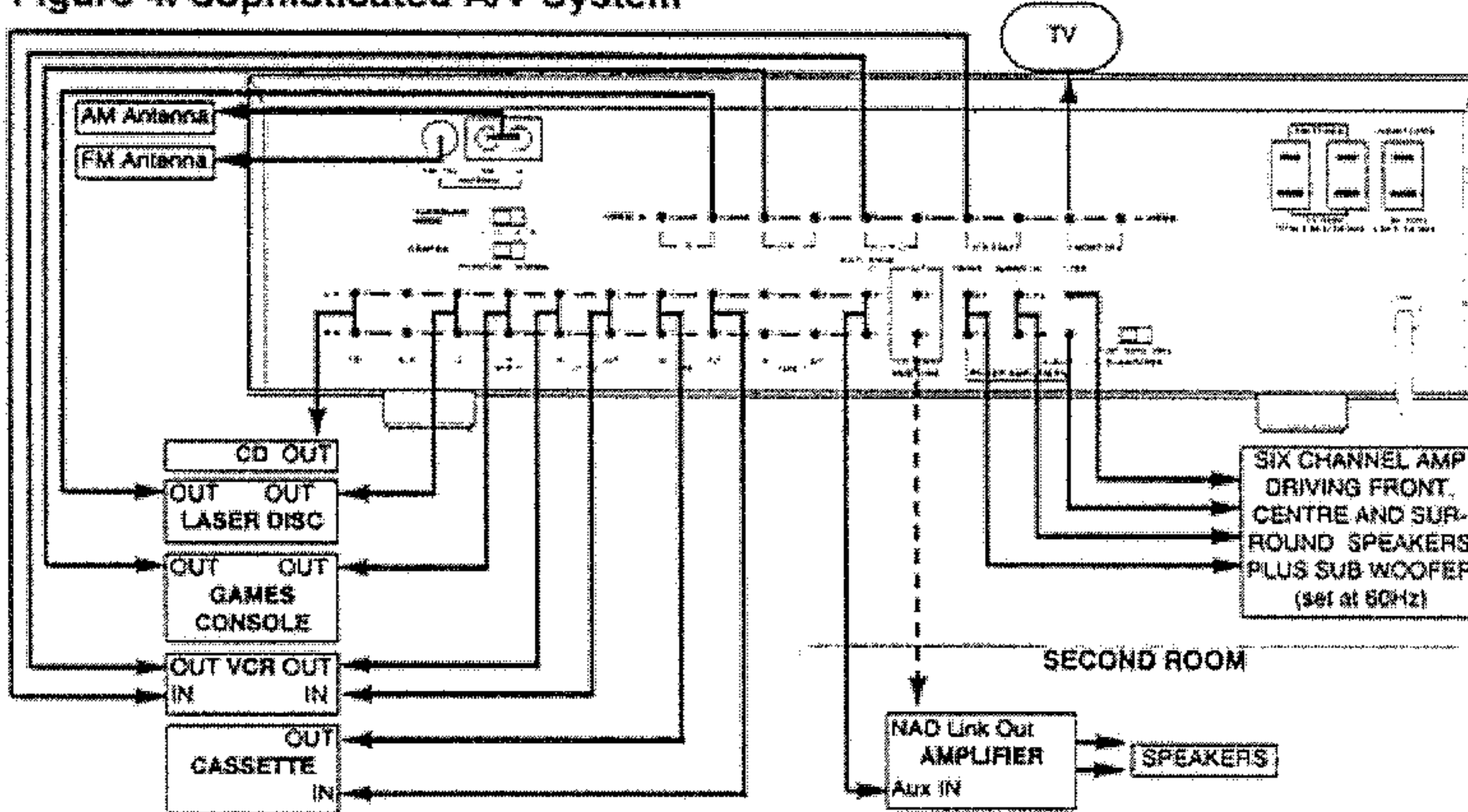
Figure 4. Sophisticated A/V System
